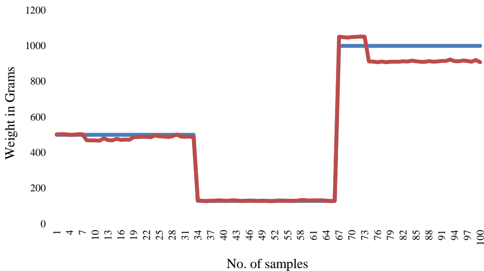
Fig. 9. Weight reading comparison of the system
