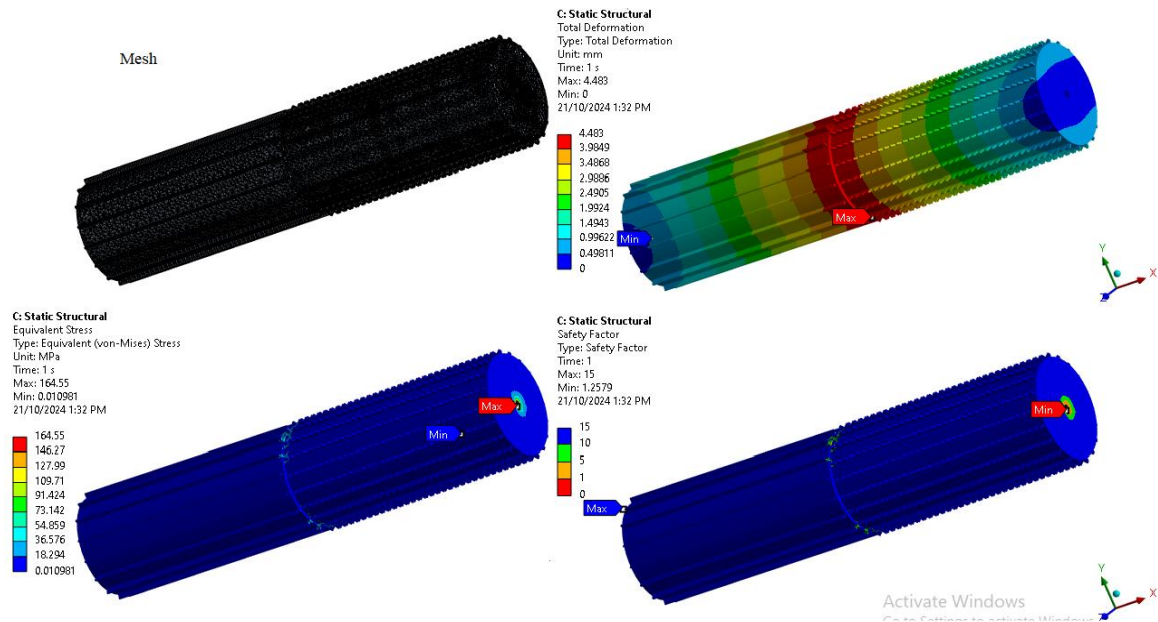
Fig. 6. Static structural analysis of the cylindrical drum
