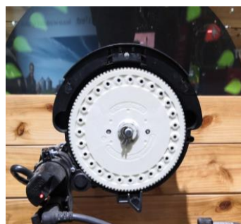
(a) Vacuum-Aspirated Precision Seed Metering Device
