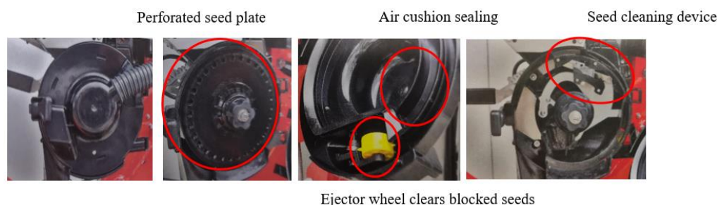
Fig. 4. Horsch vacuum-aspirated precision seed metering device
