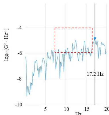
High speed, with isolator (f: 0-20 Hz)
