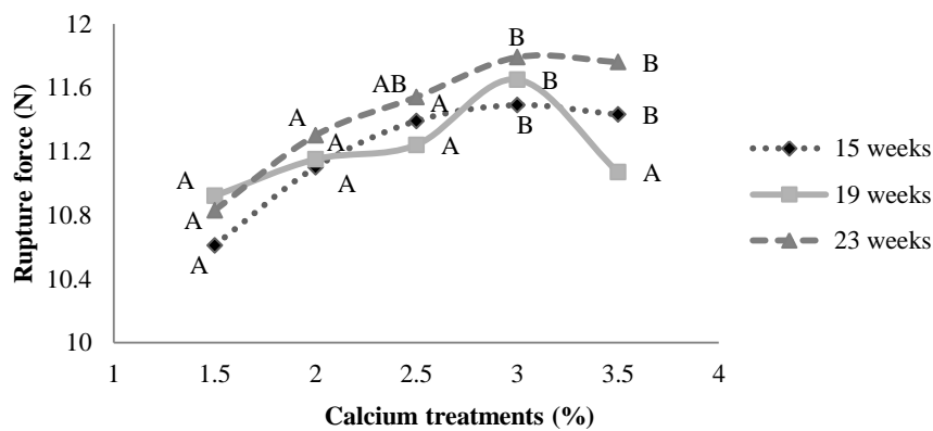
Fig.4. Changes in Rupture Force at various levels of calcium
