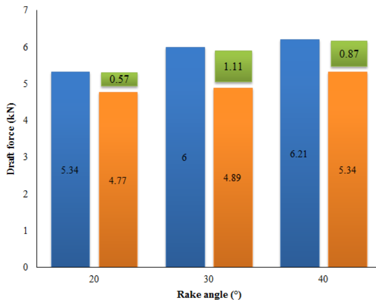
Fig.5. Comparison between the draft force of steel blade and FRP composite blade at different rake angles (blue rectangle: steel blade; orange rectangle: FRP composite blade; green rectangle: difference between steel blade and FRP composite blade)
