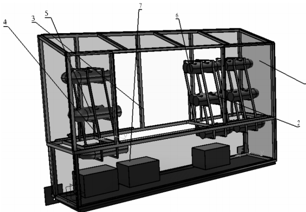
Fig. 1. System illustration: 1) Polycarbonate sheets, 2) Hydroponic pots, 3) Polymethyl Methacrylate (PMMA) sheet, 4) Pipe bases, 5) U-shaped PVC pipes, 6) The displacement subsystem, 7) Solution storage tank
