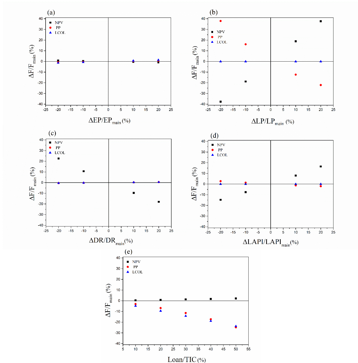
Fig. 7. Sensitivity analysis of the NPV, PP, and LCOL based on (a) EP, (b) LP, (c) DR, (d) LAPI, and (e) Loan/TIC (True Interest Cost) (%)
