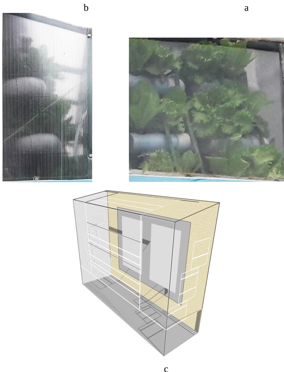
Fig. 4. Segmentation of the external cover of the novel system for precise positioning of window shadings in plant simulation: a) side view, b) front view, and c) 3D CAD
