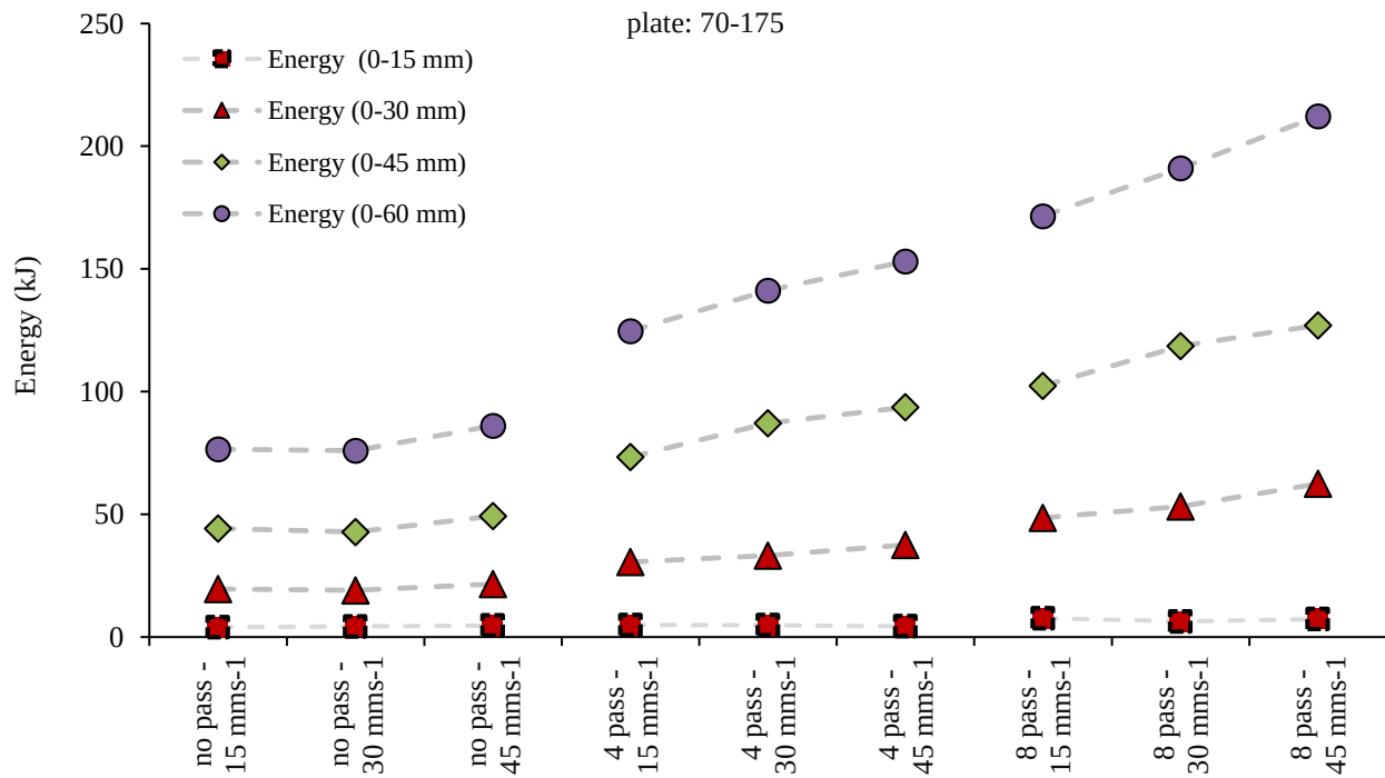
Fig. 10. The effect of penetration velocity on energy consumption in constant traffic in specified intervals, and constant traffic on the 70 × 175 plate
