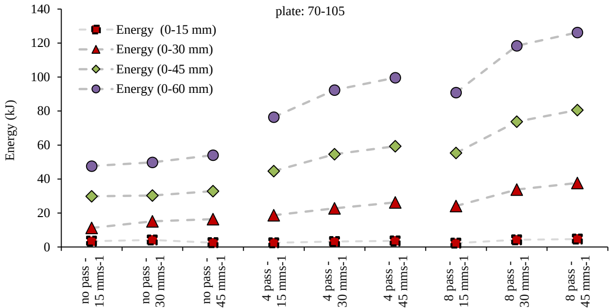
Fig. 9. The effect of penetration velocity on energy consumption in constant traffic in specified intervals, and constant traffic on the 70 × 105 plate
