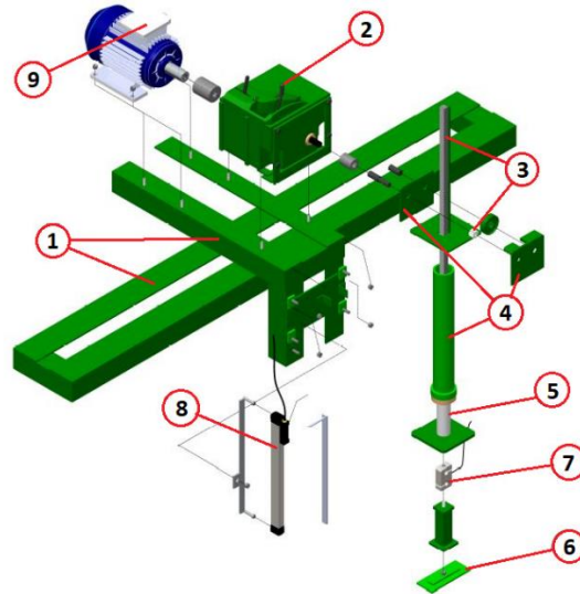
Fig. 4. Construction of the bevameter unit for soil characterization: 1. Chassis, 2. Gearbox, 3. Rail, 4. Support and Guide, 5. Shaft, 6. Bekker Plate, 7. Load cell, 8. Linear Encoder, and 9. 5.5 kW electromotor
