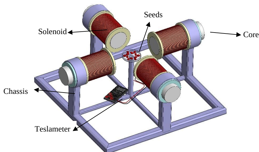
Fig. 1. Quadrupole magnetic field
