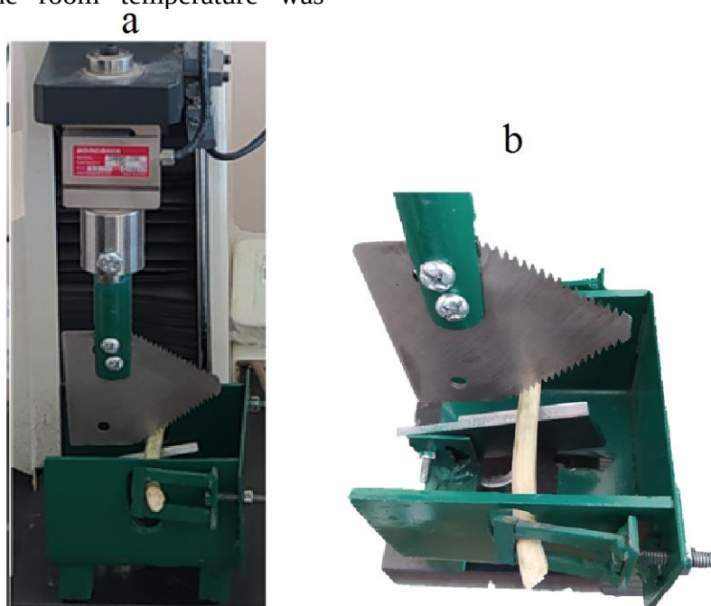
Fig. 4. A mechanism designed for conducting quasi-static tests: (a) an Instron equipped with a blade and counter blade mechanism, and (b) the blade and counter blade mechanism
