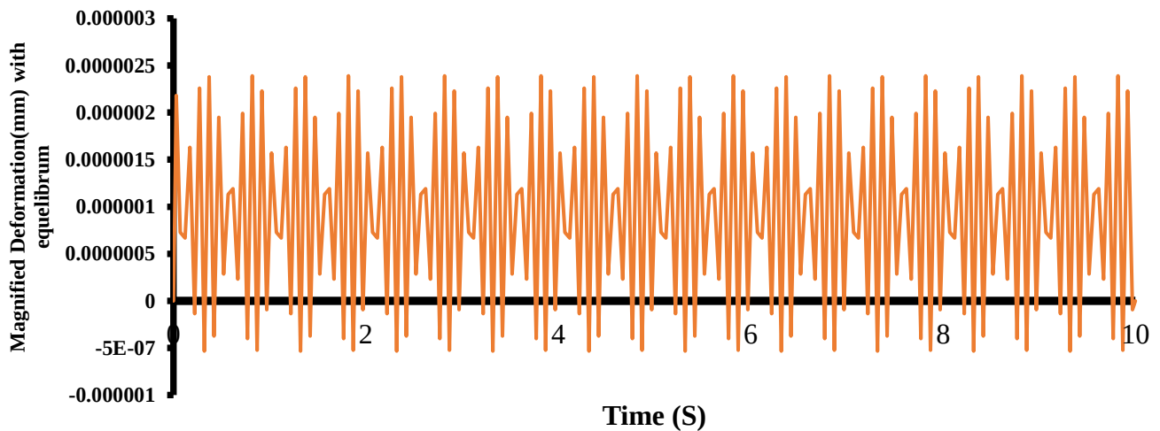
Fig. 11. Magnified directional deformation of the cylinder drum under applied dynamic load
