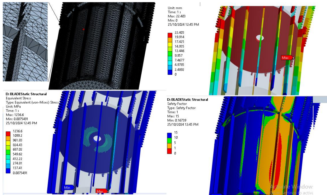
Fig. 8. Static structural analysis of the cylindrical drum's blade
