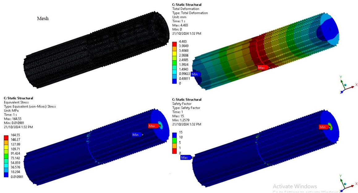
Fig. 7. Static structural analysis of the cylindrical drum
