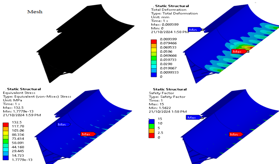
Fig. 9. Static structural analysis of the breastplate
