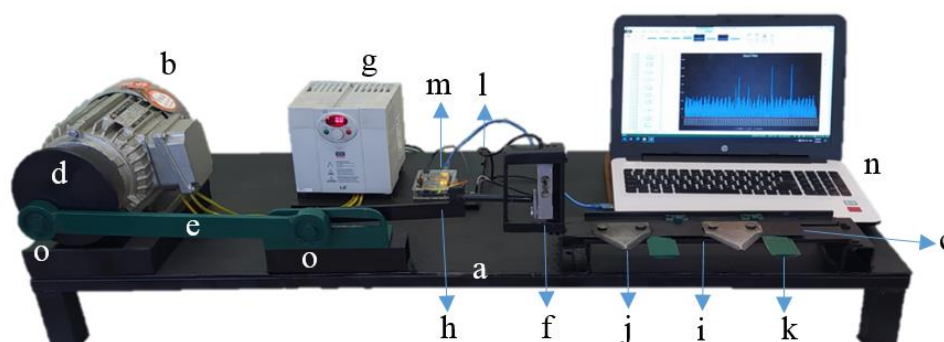
Fig. 1. The fabricated laboratory cutter bar: (a) Chassis, (b) Electric motor, (c) Upper bar, (d) Reluctance center crank drive, (e) Crank drive shaft, (f) Load cell, (g) Inverter, (h) Connecting rod, (i) Lower bar, (j) Cutting blade, (k) Designed blade, (l) HX711 amplifier module, (m) Arduino board, (n) Computer, and (o) Bearing
