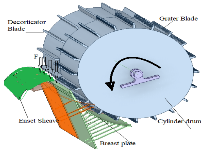
Fig. 10. Cylinder drum with breastplate
