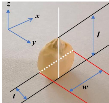
Fig. 1. Maize seed dimensions (length, width, and thickness), and digital caliper
