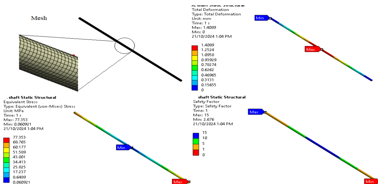
Fig. 6. Static structural analysis of shafts
