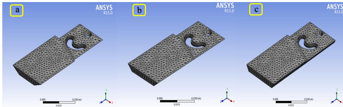
Fig. 2. Meshed models of three different designed blades: (a) the 30-degree blade, (b) the 45-degree blade, and (c) the 60-degree blade
