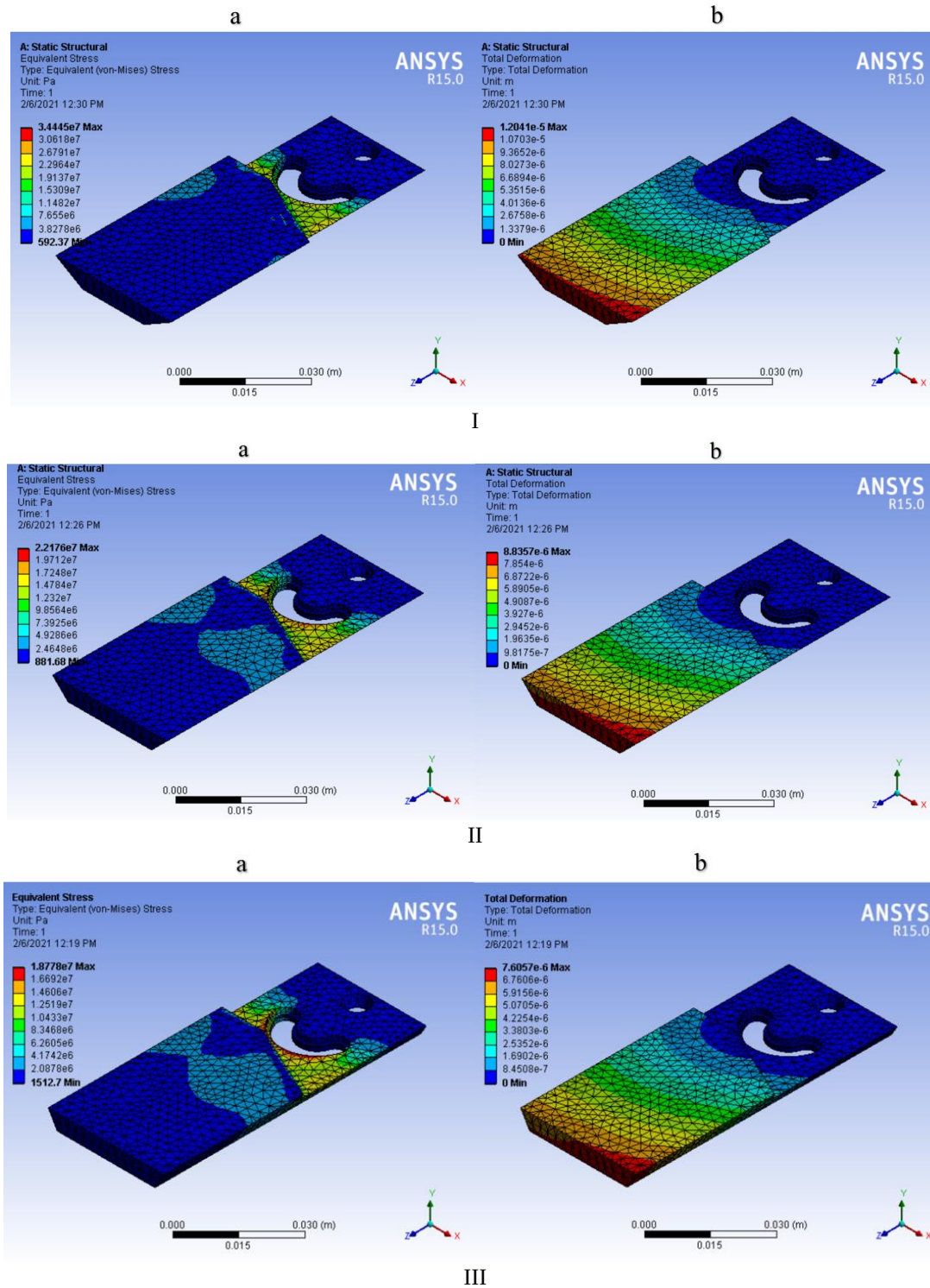
Fig. 5. Finite element analysis of the blades with sharpness angles of 30, 45, and 60 degrees (labeled I to III, respectively) under a 350 N force includes: (a) stress analysis, and (b) deformation analysis
