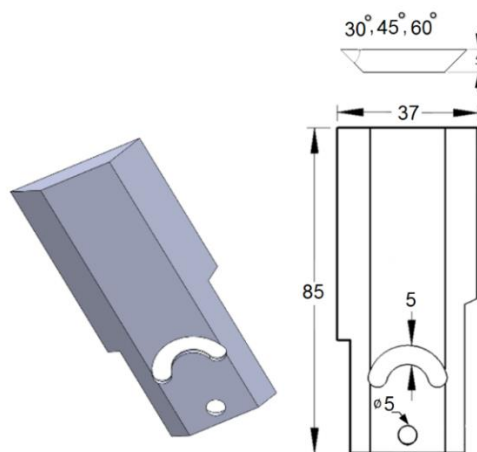
Fig. 3. Schematic of the designed blades (dimensions are in mm)
