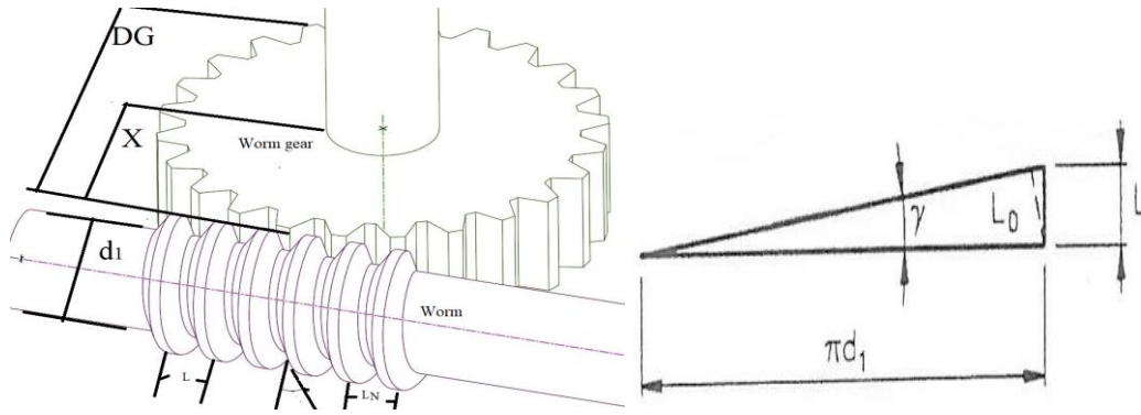
Fig. 3. Worm and gear when meshing
